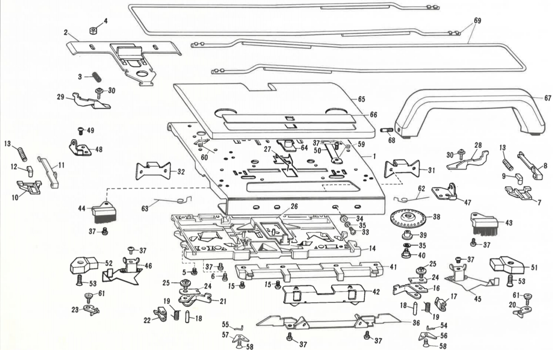
PARTS FOR L-CARRIAGE
