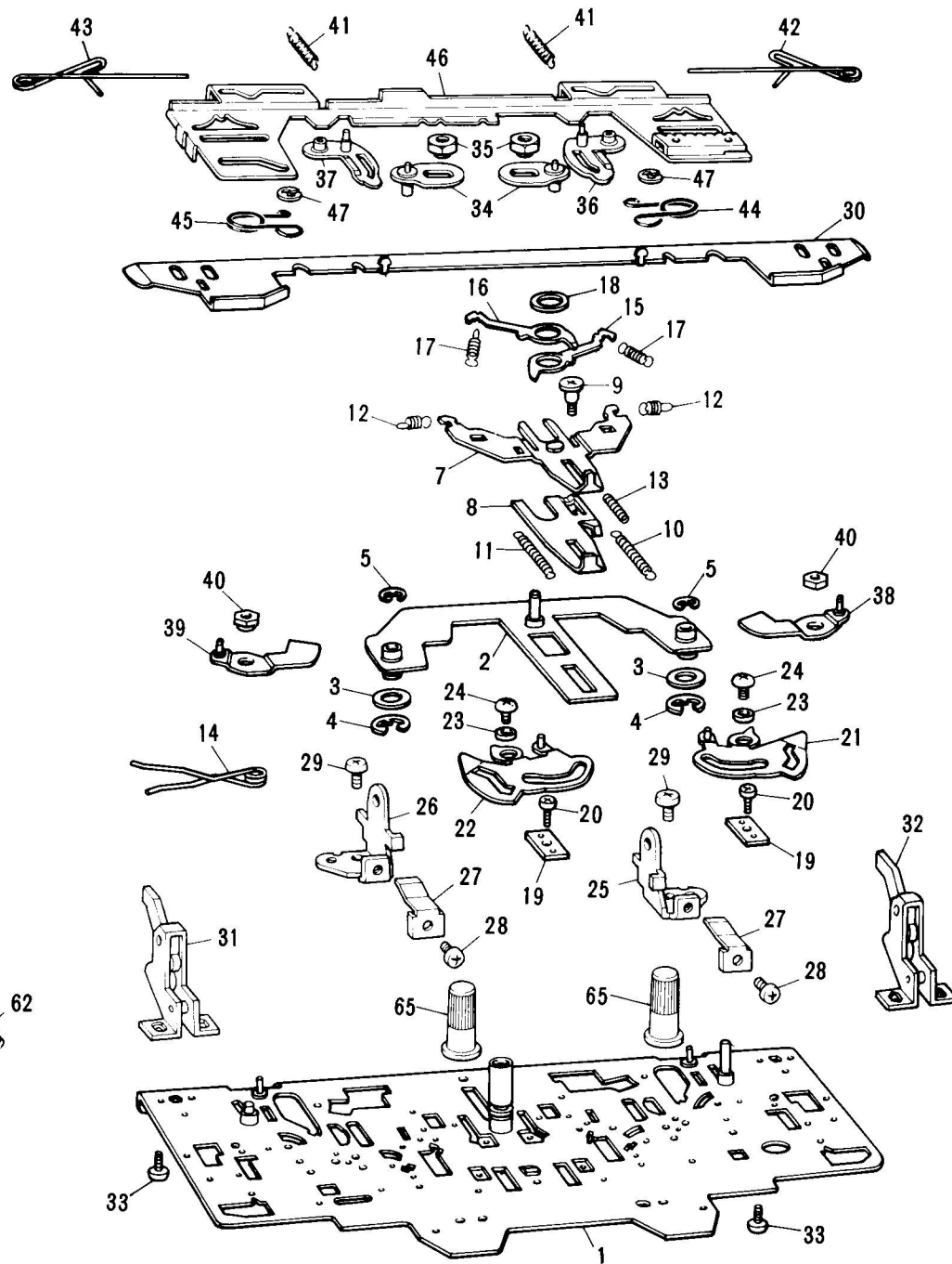
PARTS FOR CARRIAGE Fig: A I
